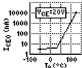
COLLECTOR DARK CURRENT -v- AMBIENT TEMPERATURE V_{CE}=20\text{V}
