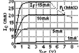
COLLECTOR-EMITTER VOLTAGE -v- COLLECTOR CURRENT T_A=25^\circ\text{C}
