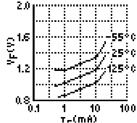
Forward Voltage (Typ) of the Diode vs Forward Current
