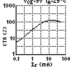
CTR vs Diode Forward Current
